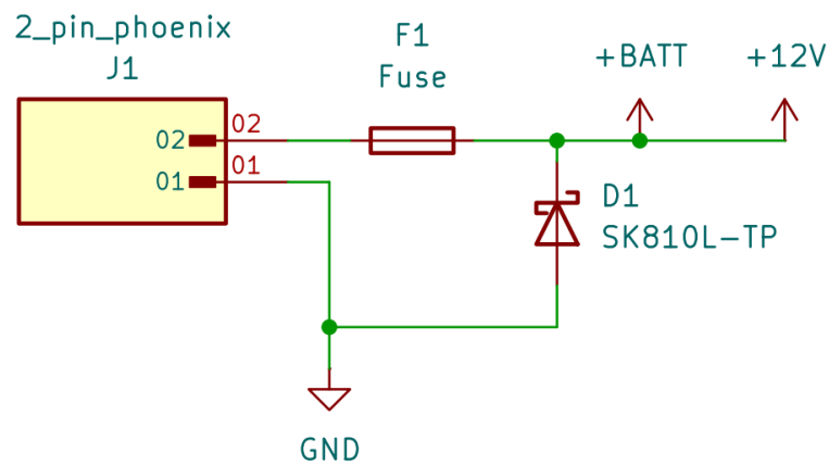
Figure 5. Power input connection schematic
