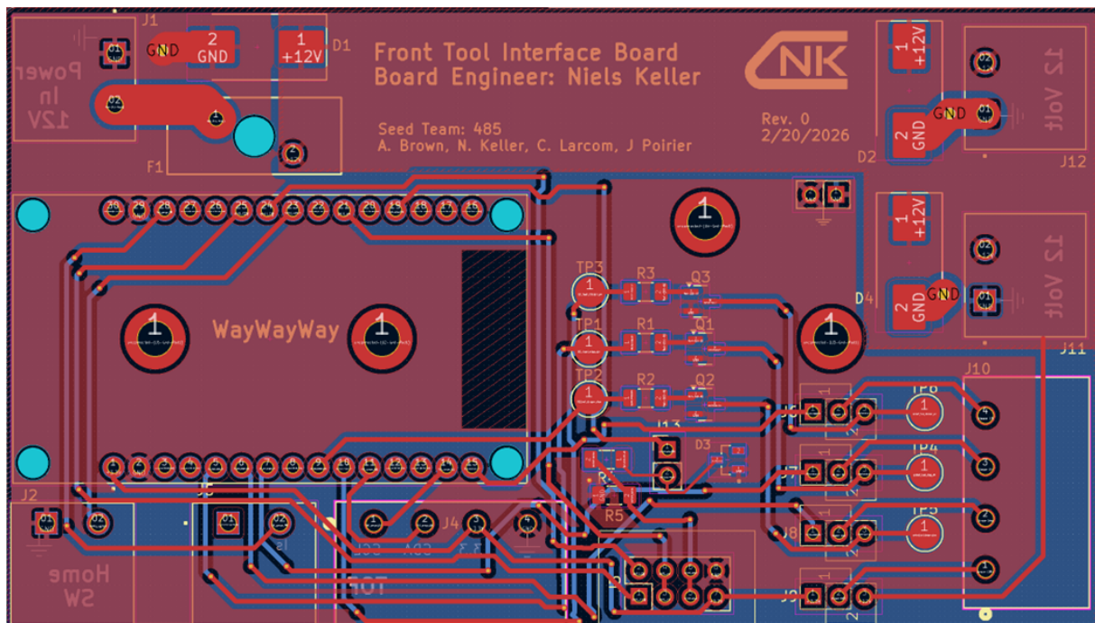
Figure 4. Front Tool PCB
