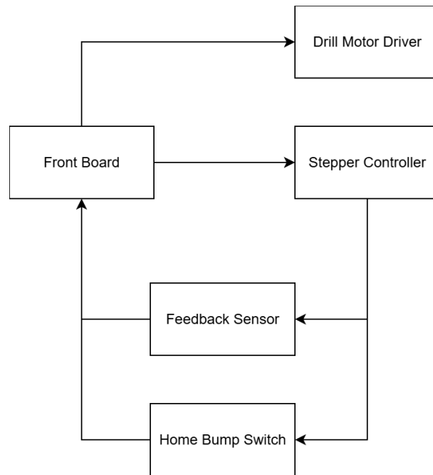
Figure 7. Front Tool System Diagram
