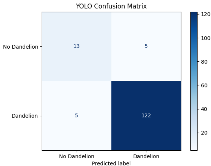
Figure 12. YOLO Confusion Matrix
