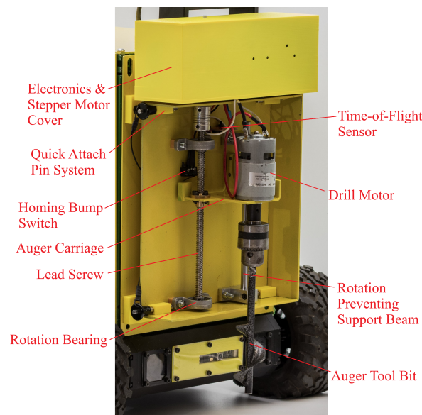
Figure 2. Auger Tool Mechanical Design
