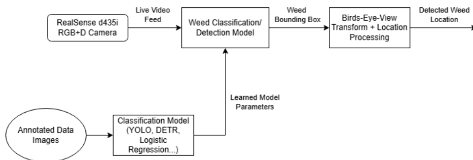
Figure 8. Machine Vision and Machine Learning System Diagram
