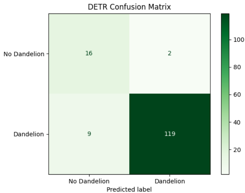
Figure 13. DETR Confusion Matrix
