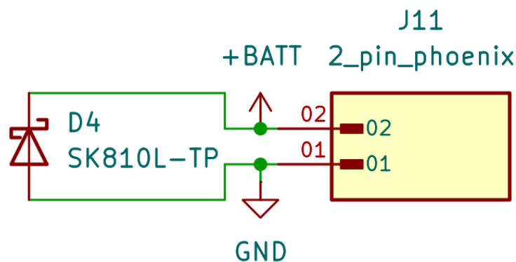
Figure 6. PCB power output schematic
