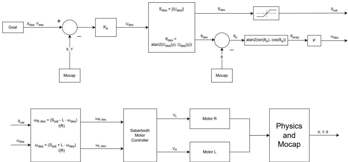
Figure 1. Go-To-Goal System Block Diagram
