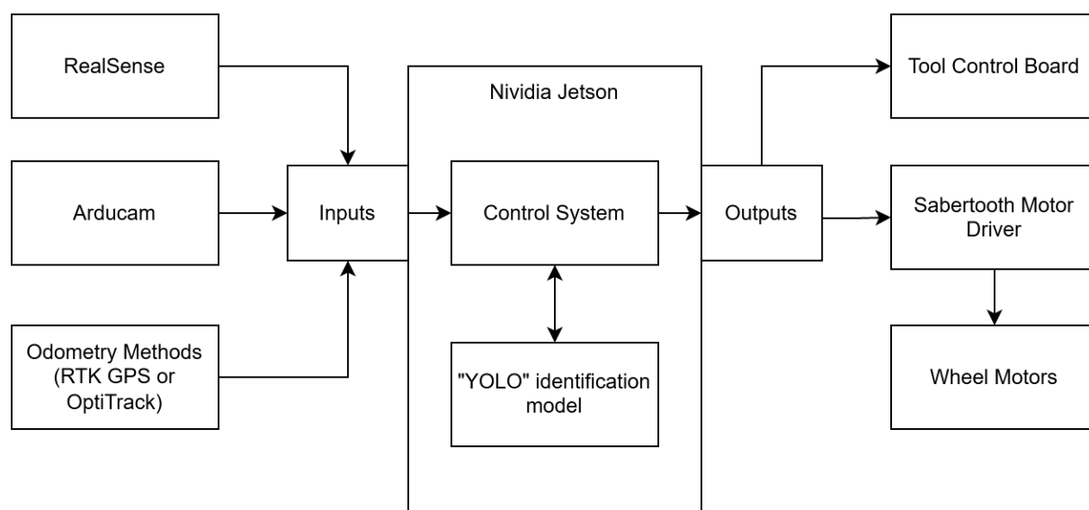
Figure 10. Full System Overview Diagram
